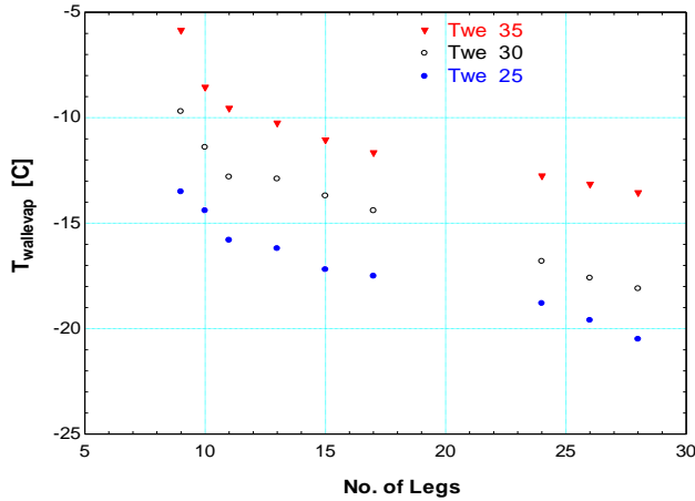
Figure 7. Evaporator wall temperature via different sizes of condensers at 25°C, 30°C and 35°C ambient temperatures.
