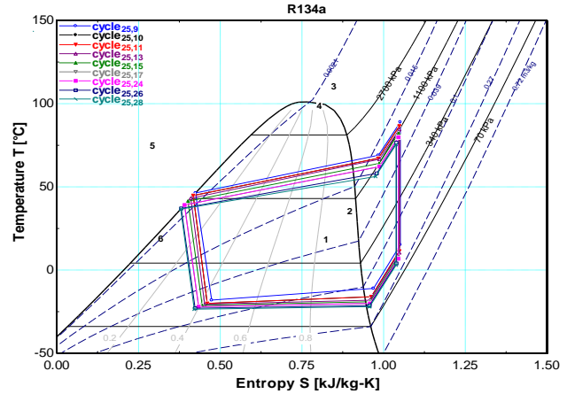
Figure 2. T-s diagrams of vapor compression refrigeration cycle with different sizes of condensers at 25°C ambient
