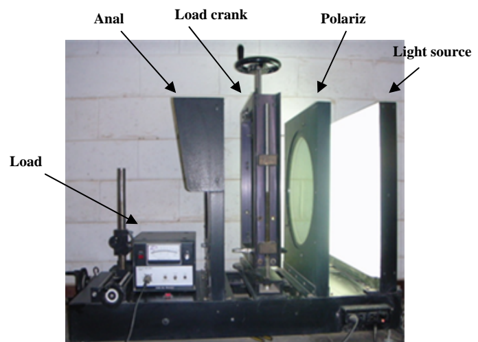
Fig.5 Experimental Apparatus
