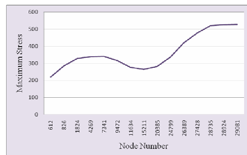
Fig. 1 Convergence test
