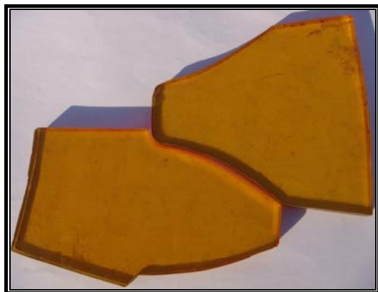
Fig. 4 Splined Shaft Photoelastic Models
