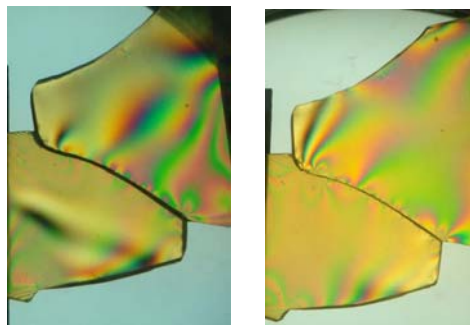
Fig. 14 Results of photoelastic fringes show the contact and bending stresses for two load cases of spline teeth .
