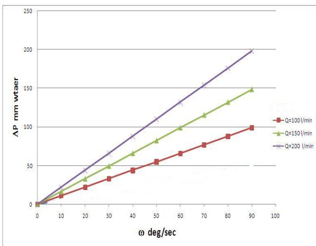
Figure.6 Theoretical static characteristics.
