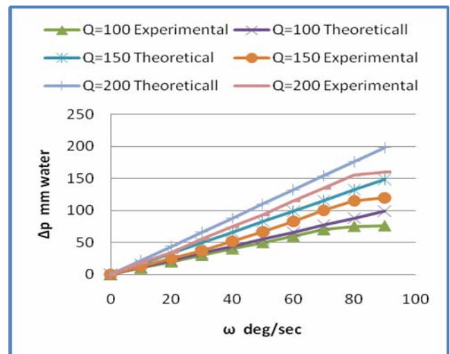
Figure.8 Comparison between theoretical and experimental static characteristics.
