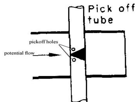
Fig.2 Schematic of Cylindrical Pickoff Element
