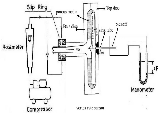
Fig.3 Testing Rig
