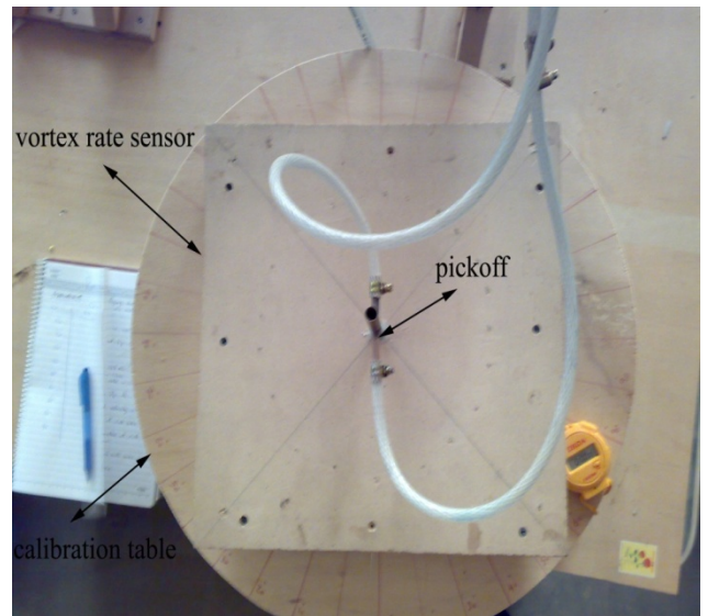
Fig.4 pickoff tube used in the test rig
