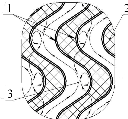
Figure 6. the gas fluid movement along the separation board of the IF drop catcher scheme: 1 – double louver crimped plate made of net, 2 – filtering element, 3 – gas fluid flow.
