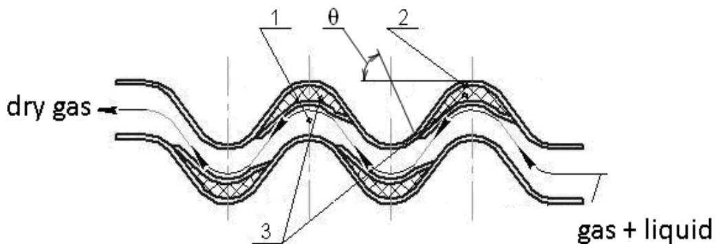
Figure.2. Calculating scheme of the gas liquid drop flow movement along the separation channel with filtering sections IF separation apparatus: 1. - separation channel; 2- double louver crimping plates; 3- filtering sections.
