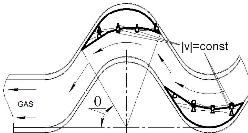
Figure.4. Geometrical zones of the filtering sections in the separation channel of the louver inertial filtering gas separator disposition. ( Re \geq 10000 ).
