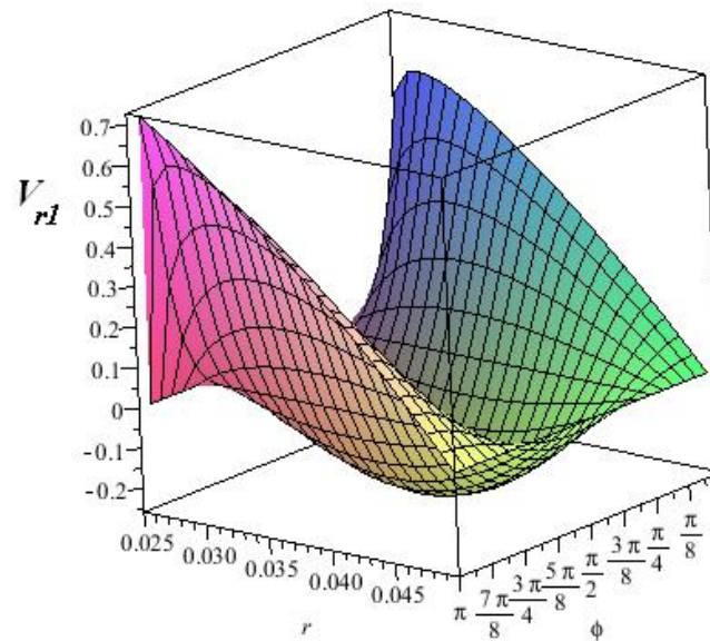
Figure.5. The example of the graphic results for calculation the changes of the radial component for the gas flow speed along curvilinear channel with sizes R_1=50\text{mm} , R_2=25\text{mm} and the radial component of the gas flow speed at \phi_0=0 equal to V_{r1}=1 m/sec.
