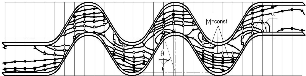
Figure.3. Local speeds distribution.
