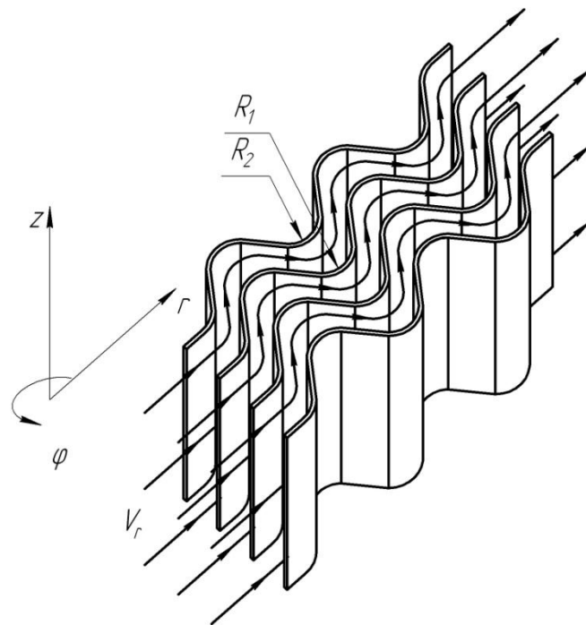
Figure. 1. The calculating scheme of the purifying gas movement through the IF separator louver board.
