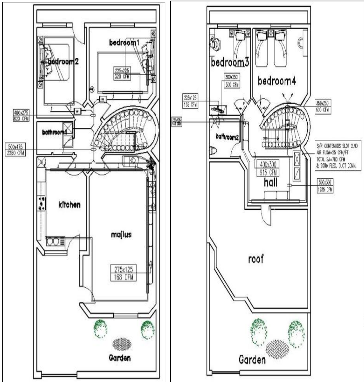
Figure 4. Air Conditioning plans layout.
