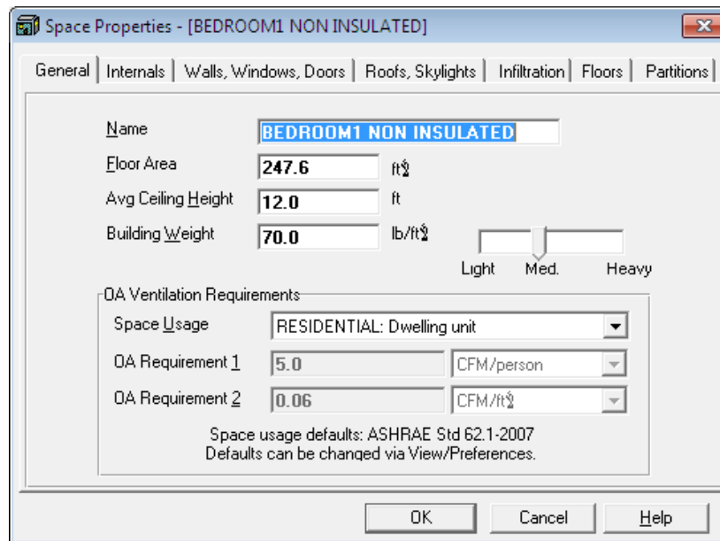
.Figure 5. HAP space properties.
