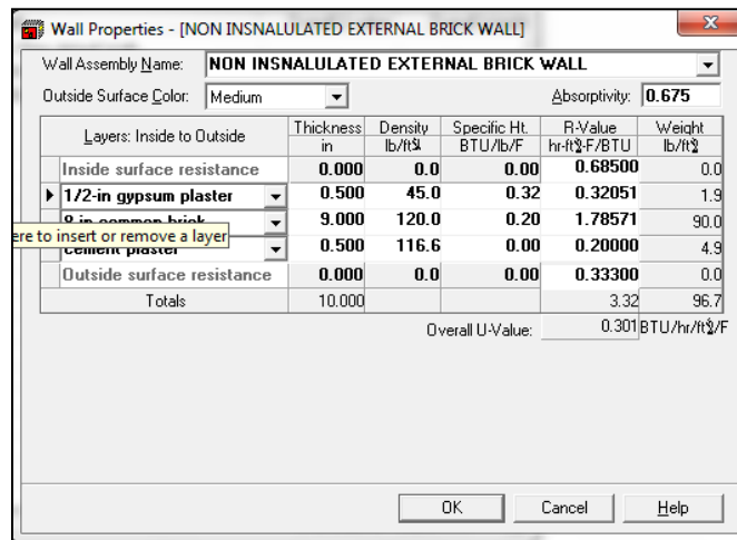
Figure 7. HAP U-Value and R-Values for Non-Insulated wall (Researcher).
