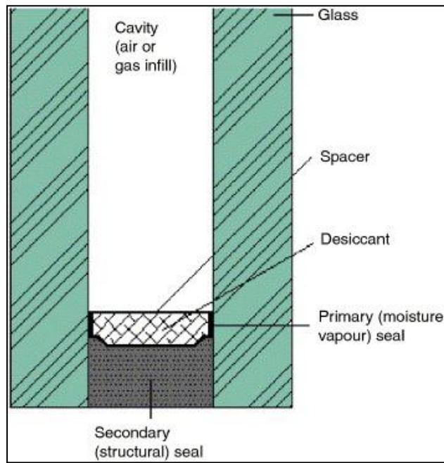
Figure 1. Cross section of a dual sealed double glazing unit, Song et al., 2005.
