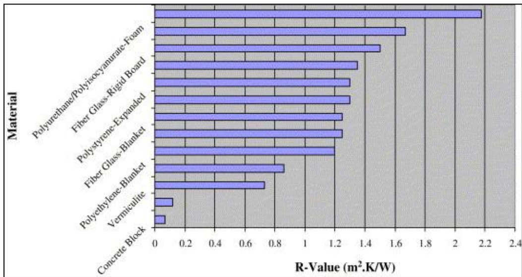
Figure 3. Thermal resistances (5cm thickness) of common building insulation materials (Concrete block is added for comparison purposes), Al-Homoud, 2004.
