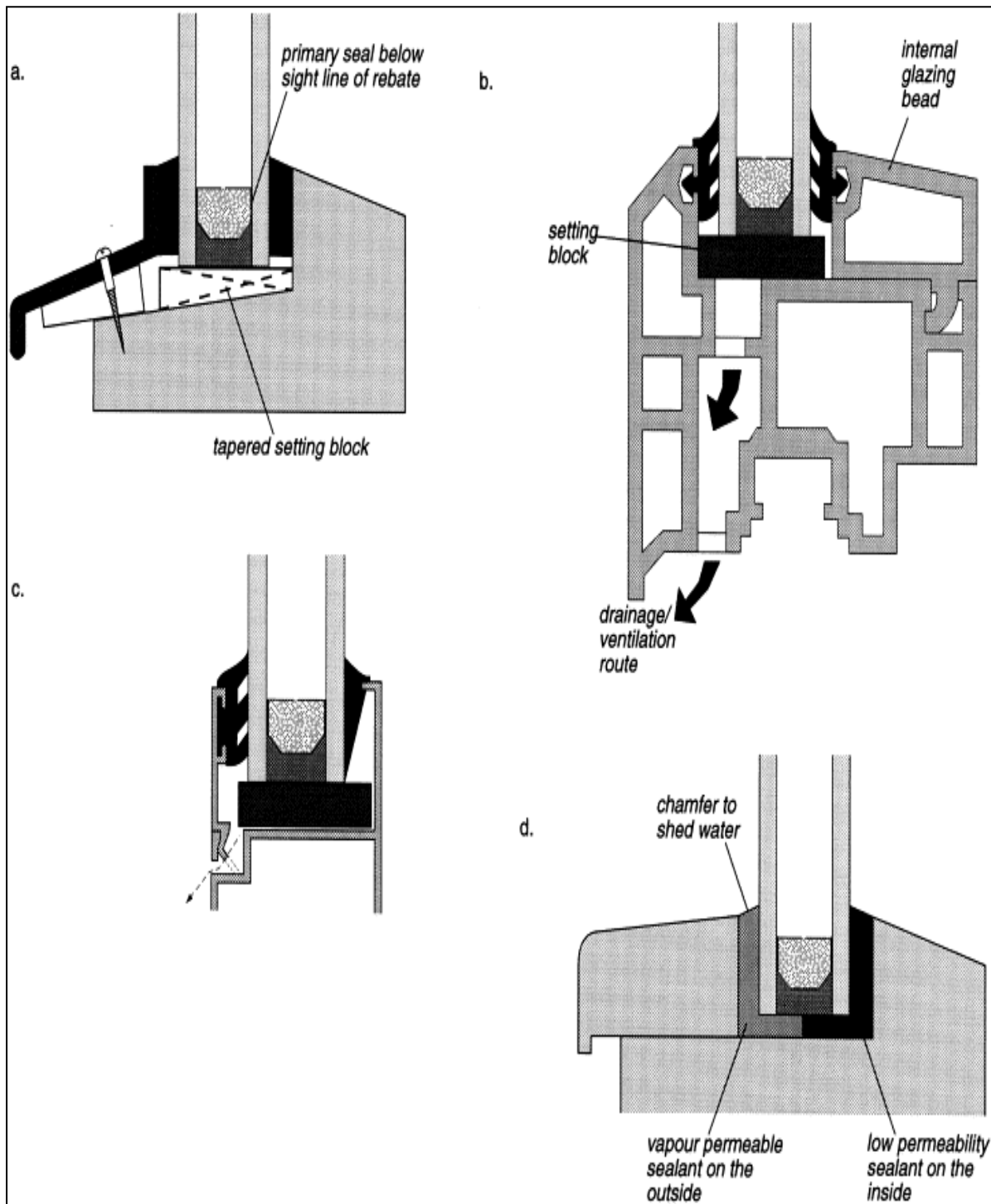
Figure 2. Drained and ventilated and fully bedded window frames. (a) Timber; (b) PVC; (c) aluminum; (d) timber fully bedded, Garvin and Wilson, 1998.
