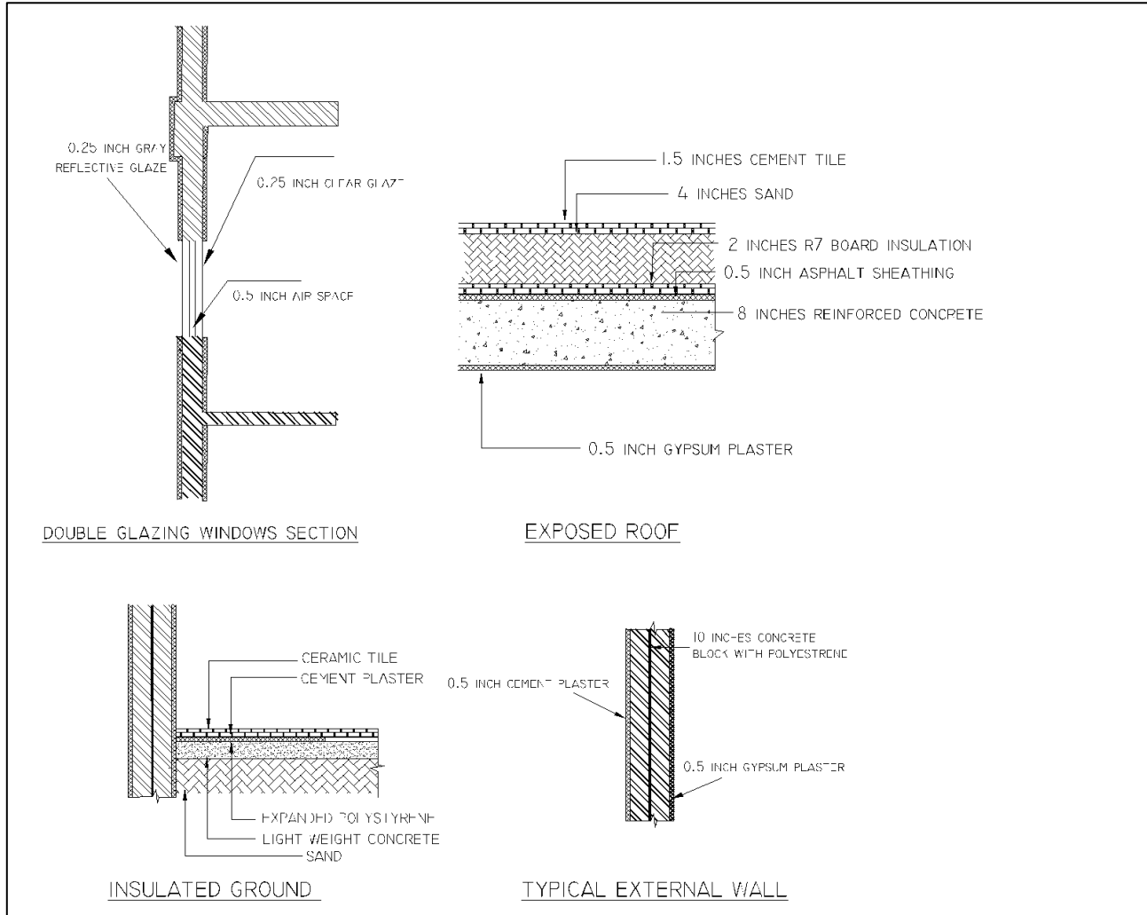
Figure 6. Insulated roofs, walls, floors, and double glazing windows (Researcher).
