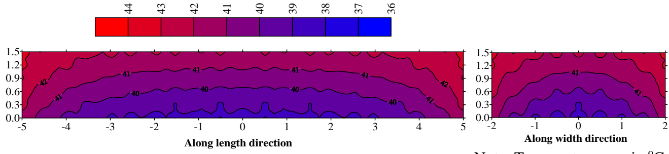
Fig. (9): Temperature distribution in a slab with B/L=0.4 (180 days after placement)
