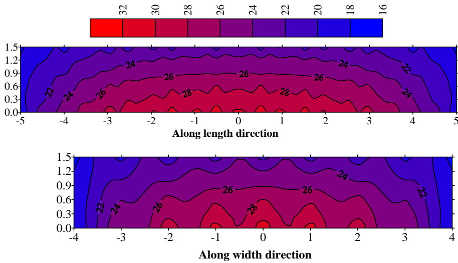
Fig. (11): Temperature distribution in a slab with B/L=0.8 (28 days after placement)
