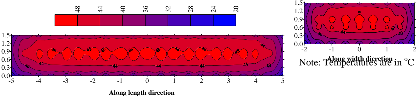
Fig. (7): Temperature distribution in a slab with B/L=0.4 (3 days after placement)
