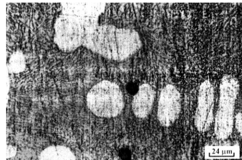
Al-12%Si-1%Pb
