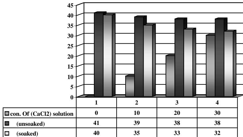
A: Variation of Cohesion (c) with c.c.s of unsoaked and Soaked Samples
