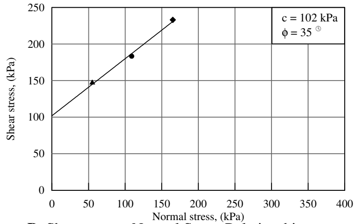
B: Shear stress -Normal Stress Relationship
