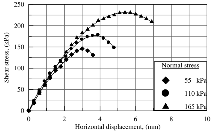
A: Shear Stress-Horizontal Displacement Relationship
