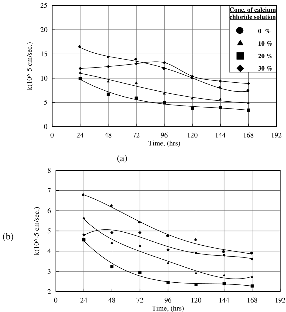
Fig. (5). Results of Oedometer-Permeability Leaching Test of Samples Treated with Different (c.c.s):
