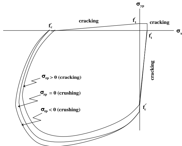
Fig.(1): Failure surface in principal stress space with nearly biaxial stress state, after ANSYS Inc.
