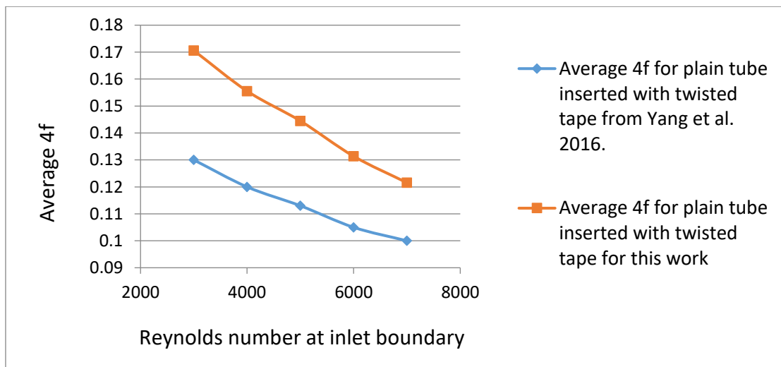
Figure 12. Comparison of average 4f computed from this work and Yang, et al., 2016.
