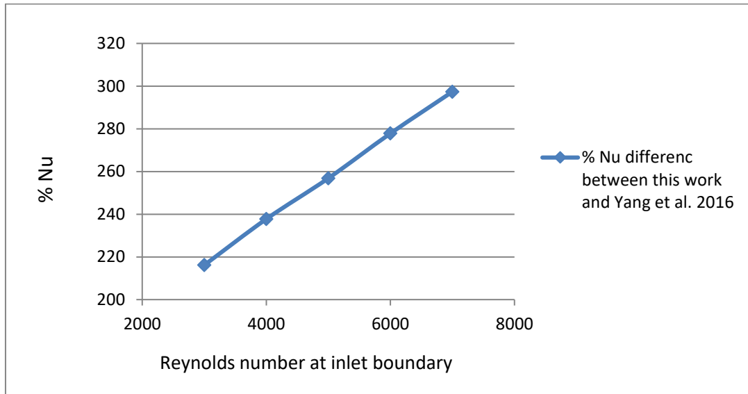
Figure 11. Percentage average Nusselt number differences with Reynolds number between this work and Yang, et al., 2016 work.
