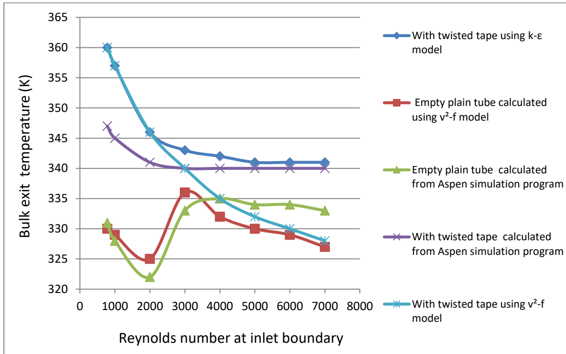
Figure 3. Bulk exit temperature of crude oil API 28 from empty plain tube and plain tube with inserted with twisted tape.
