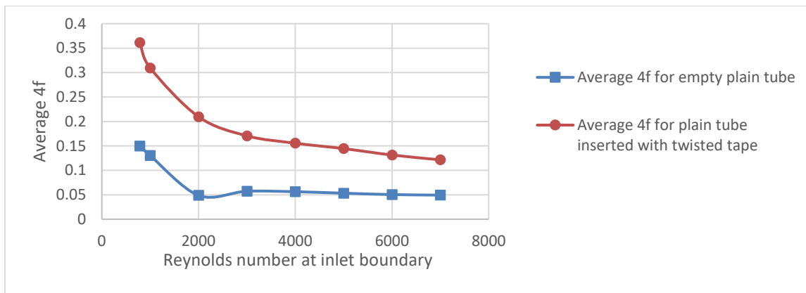
Figure 6. Variation of average tube surface friction factor with inlet Reynolds numbers for empty plain tube and plain tube inserted with twisted tape.
