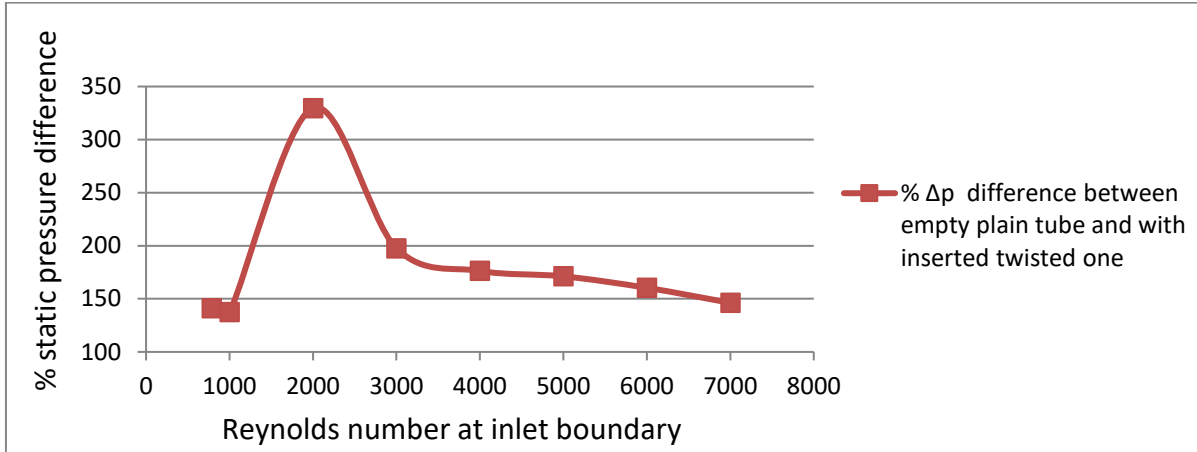
Figure 5. Variation of percentage static pressure difference increase with inlet Reynolds numbers for plain tube inserted with twisted tape over empty plain tube.
