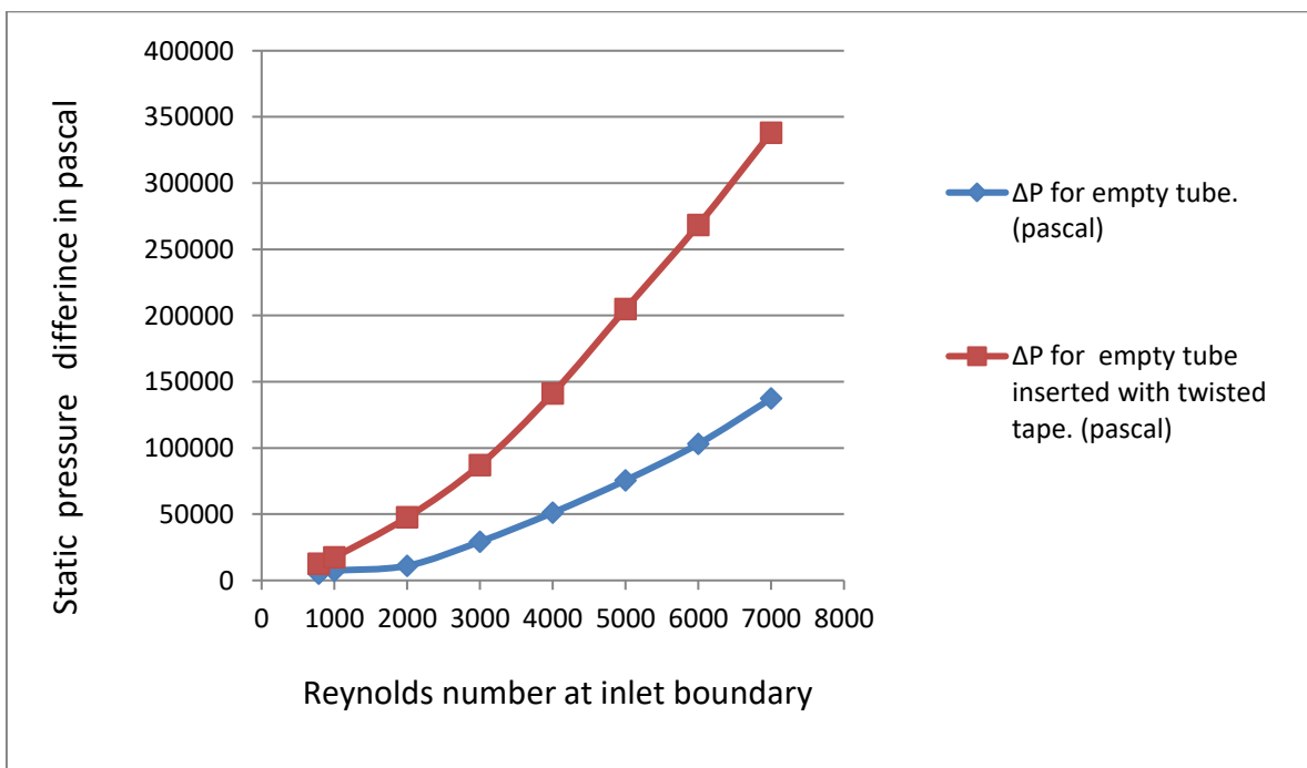
Figure 4. Variation of static pressure difference with inlet Reynolds numbers for empty plain tube and plain tube inserted with twisted tape by using ANSYS Fluent.
