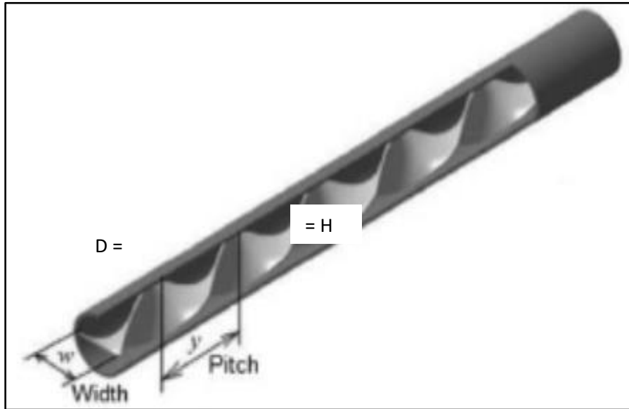
Figure 1. 3D view of tube inserted with twisted tape.
