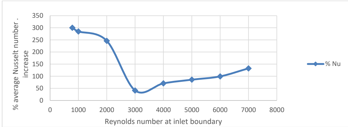
Figure 8. Variation of percentage increase of average Nusselt number with inlet Reynolds numbers for plain tube inserted with twisted tape over empty plain tube.
