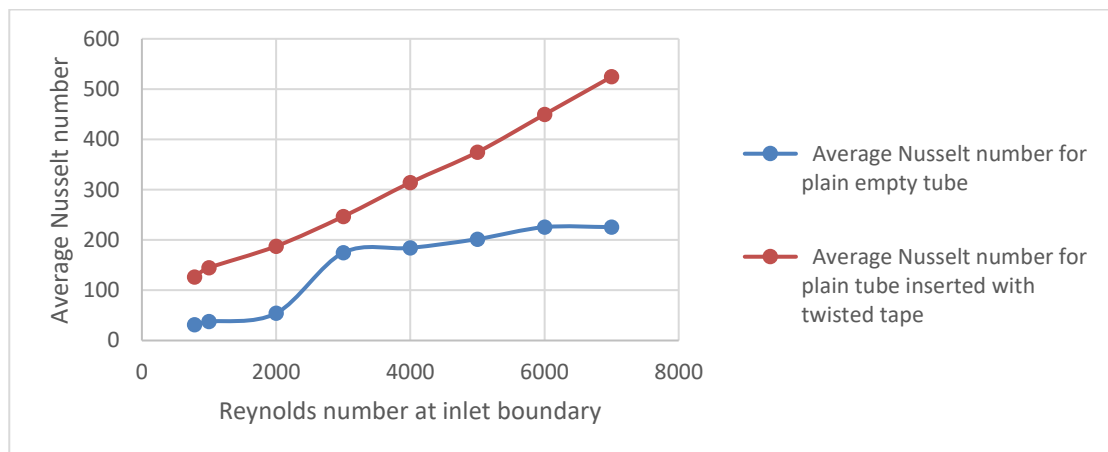
Figure 7. Variation of average tube surface Nusselt number with inlet Reynolds numbers for empty plain tube and plain tube inserted with twisted tape.
