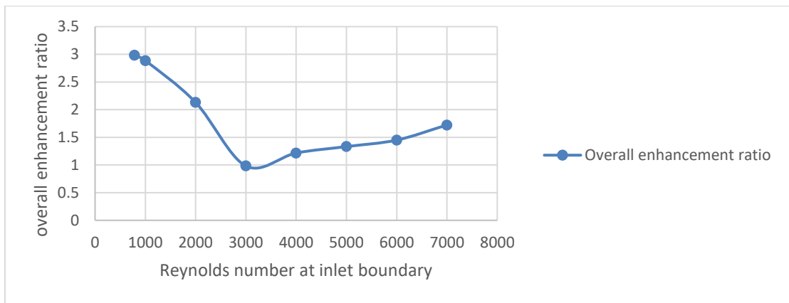
Figure 9. Variation of overall enhancement ratio with inlet Reynolds numbers for empty plain tube and plain tube inserted with twisted tape.
