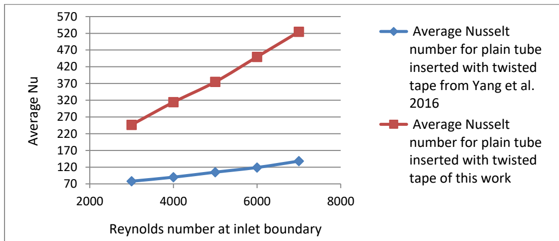
Figure 10. Comparison of average Nusselt number computed from this work and Yang et al. 2016.
