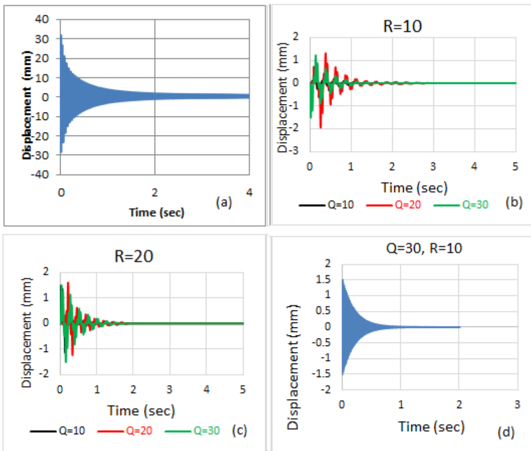
Figure 4. (a) Free vibration without active control. Results of active vibration control of experimental results shown in (b, c) while (d) show the numerical result.
