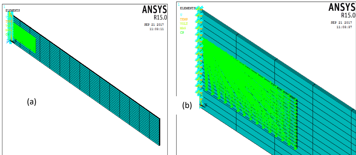
Figure 1. The finite element model of the cantilever beam embedded with piezoelectric. (a) Showing elements of the cantilever beam (b) Detail of boundary conditions and the model.
