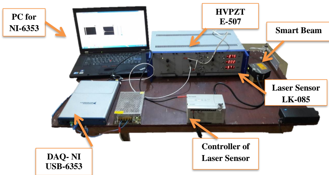
Figure 2. Experimental system.
