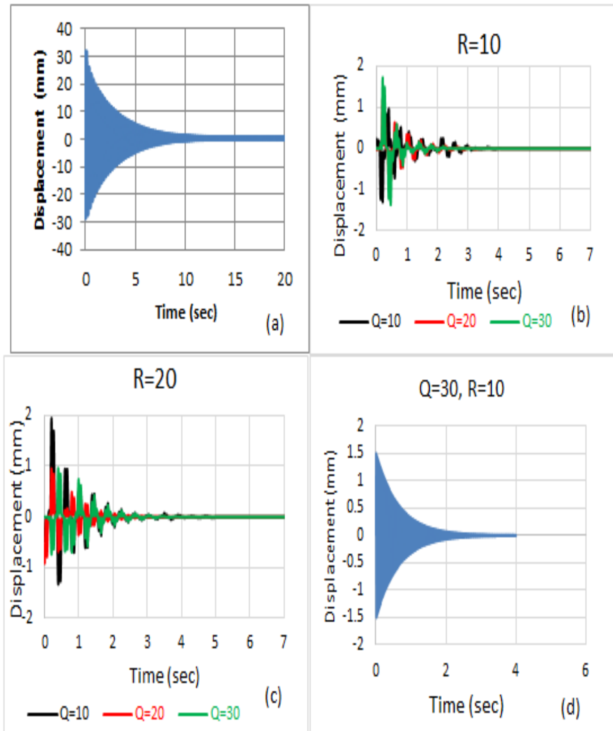
Figure 7. (a) Free vibration without active control. Results of active vibration control of experimental results shown in (b, c) while (d) show the numerical result.
