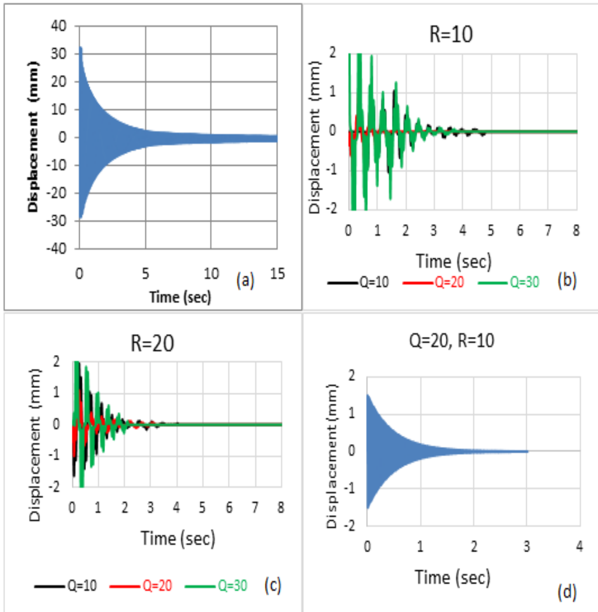
Figure 5. (a) Free vibration without active control. Results of active vibration control of experimental results shown in (b, c) while (d) show the numerical result.
