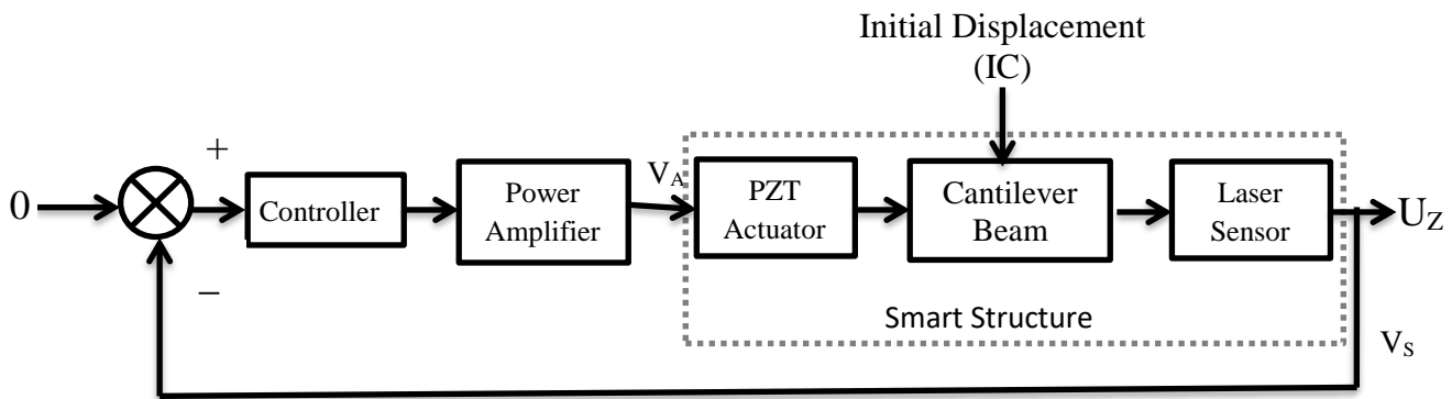
Frame. The Block diagram of free vibration analysis.
