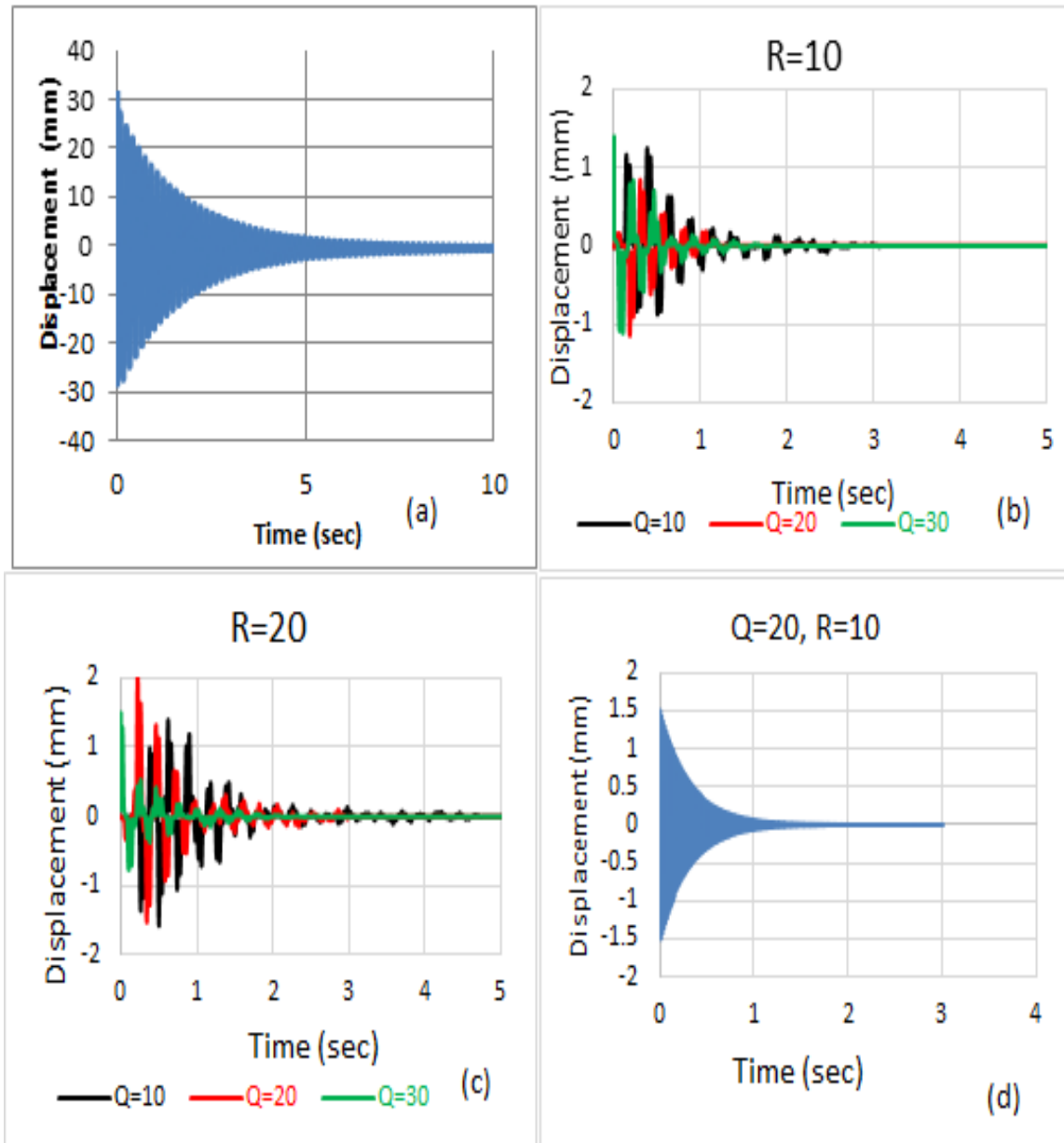
Figure 6. (a) Free vibration without active control. Results of active vibration control of experimental results shown in (b, c) while (d) show the numerical result.
